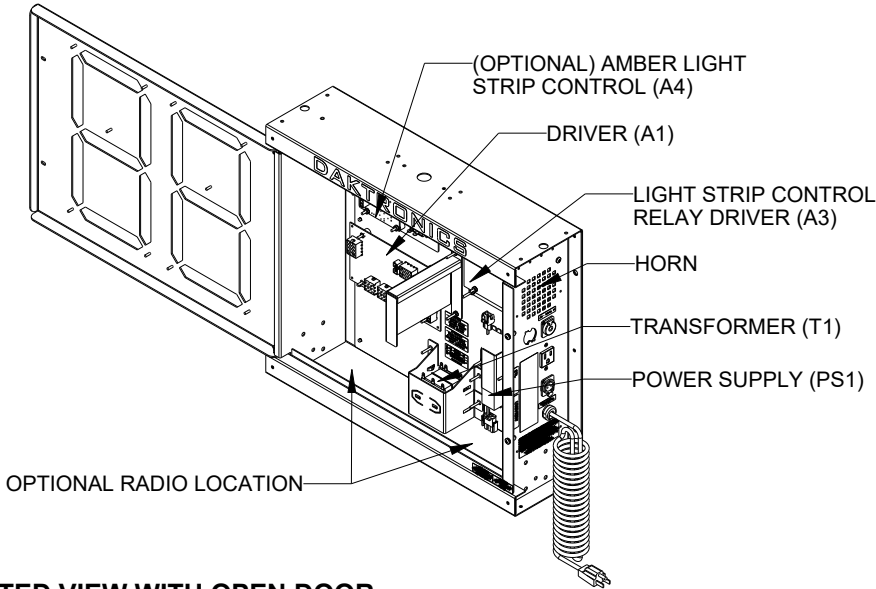
ROTATED VIEW WITH OPEN DOOR
