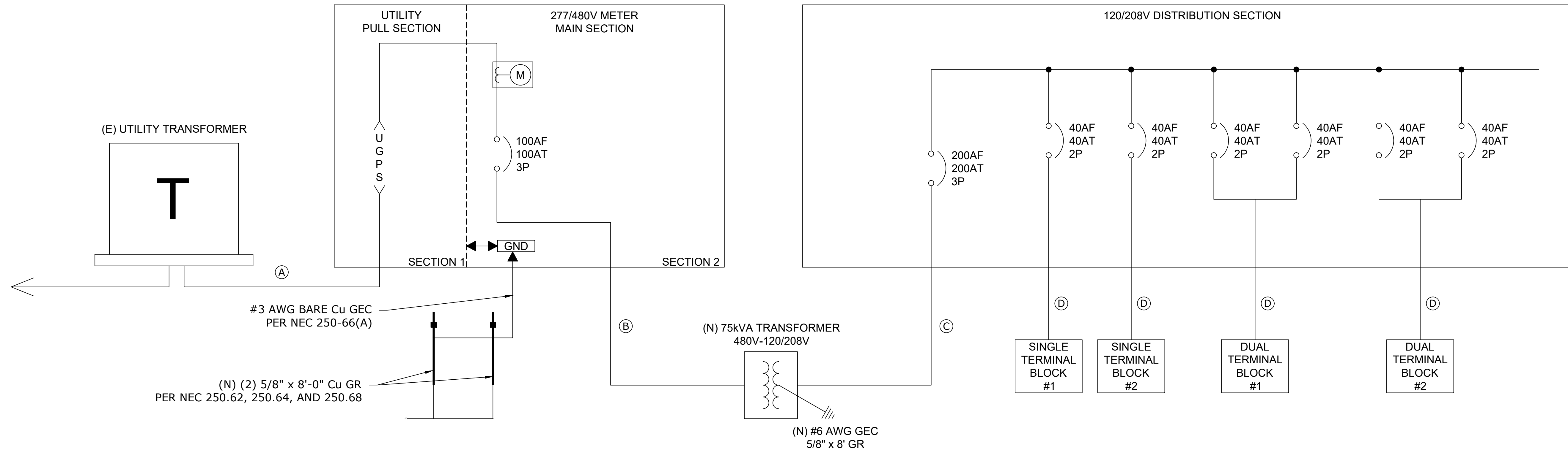
A SINGLE LINE DIAGRAM SCALE: NTS
